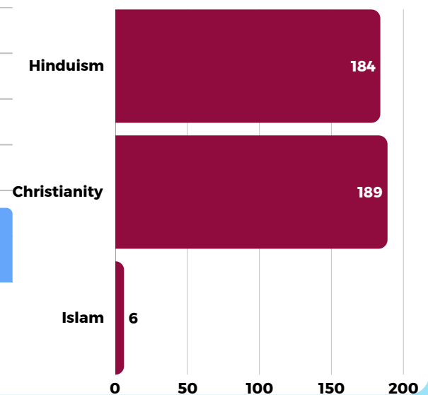
Religion Classification
