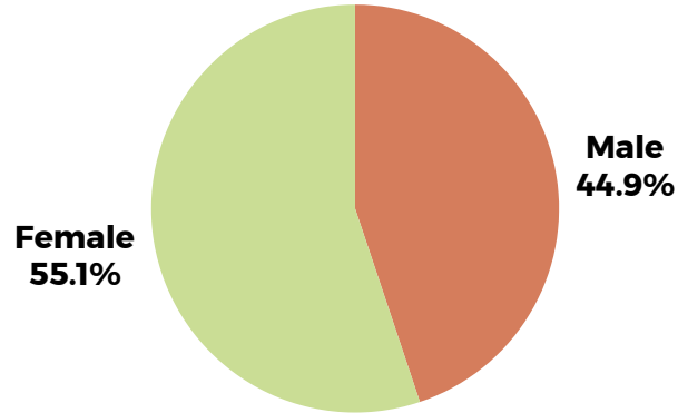
Gender Classification
