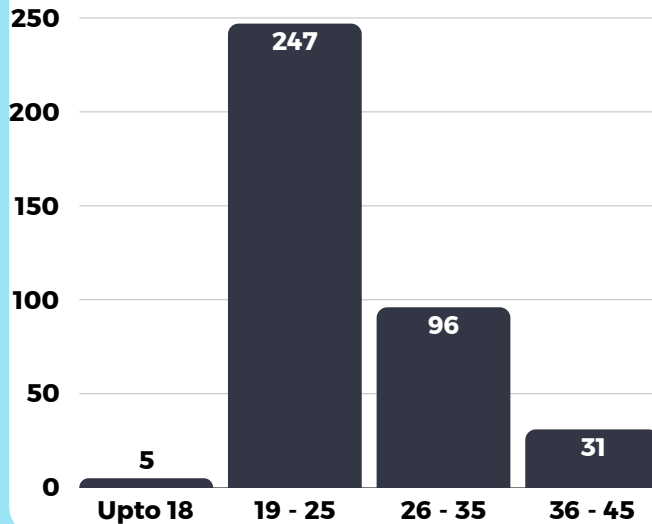
Age Classification
