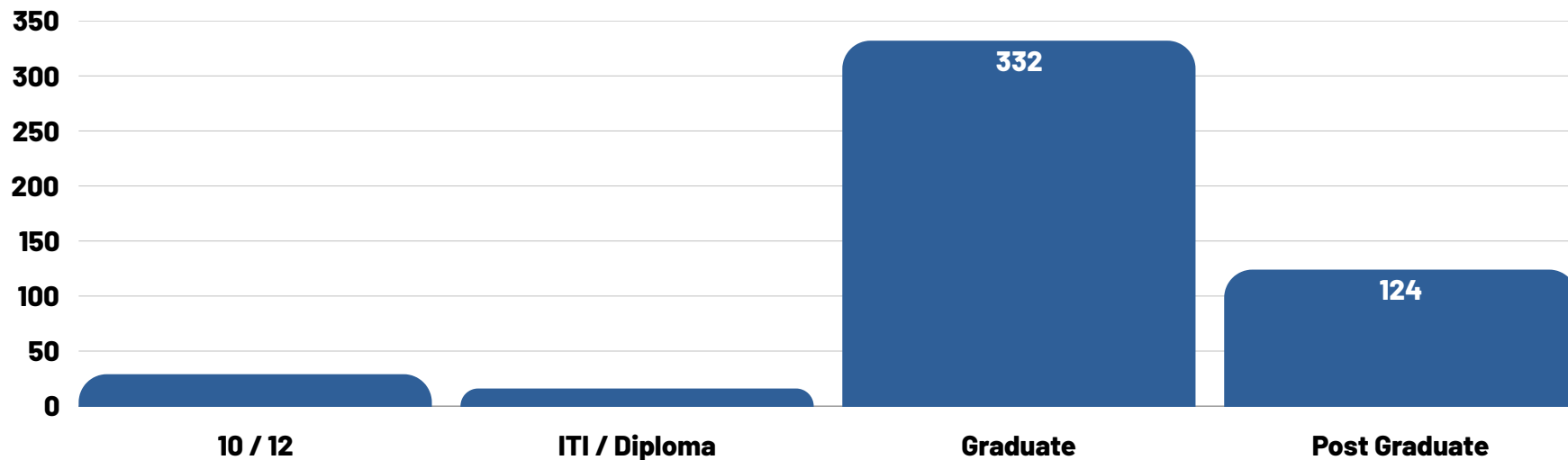
Education
