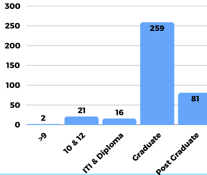
Education Classification
