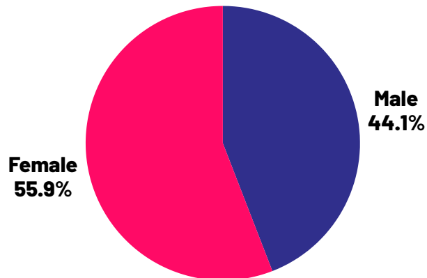
Gender Classification
