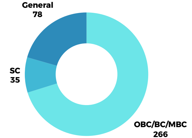
Caste Classification
